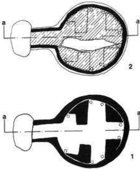
Fig. 3. Pottery kiln from Sirmium (after Premk 1993).
