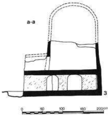
Fig. 4. Pottery kiln from Vranj (after Dautova-Ruševljan 1991).
